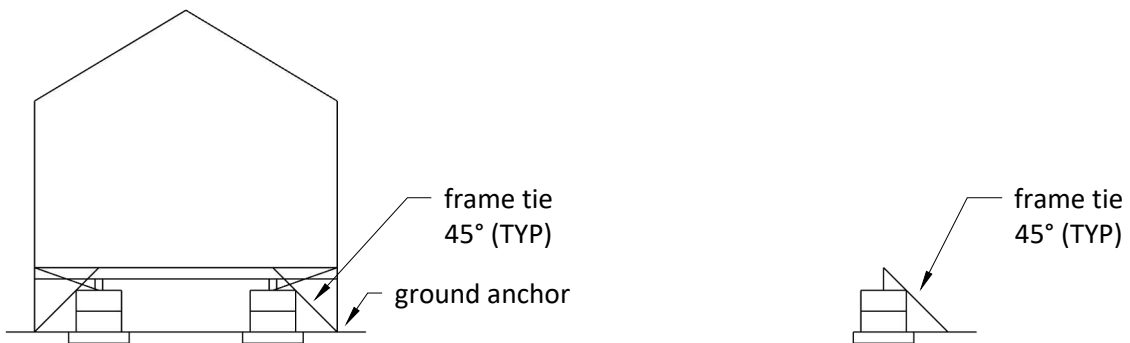
Example Elevations - Foundation and Anchorage System (as provided by manufacturer) Scale: 1:100
