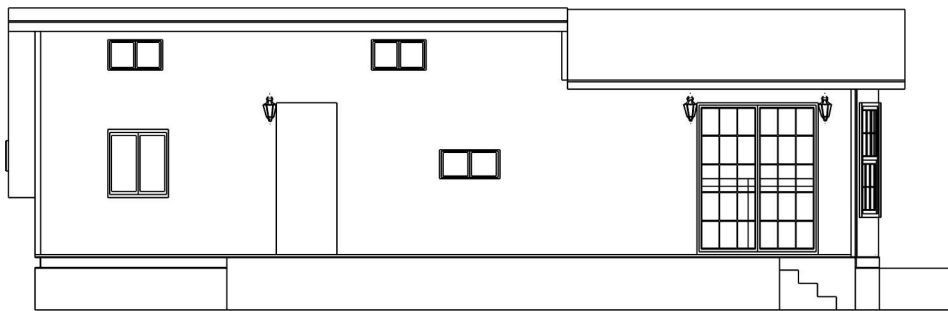
Elevation A (include windows and doors sizes) Scale: 1:100
