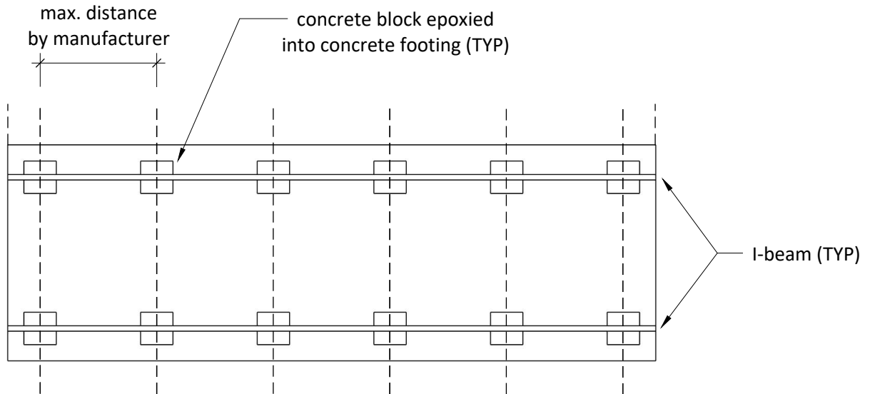
Example Floor Plan - Foundation and Anchorage System (as provided by manufacturer) Scale: 1:100
